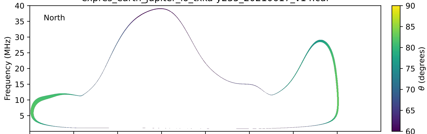
expres_earth_jupiter_io_txka-y235_20210617_v14.cdf
