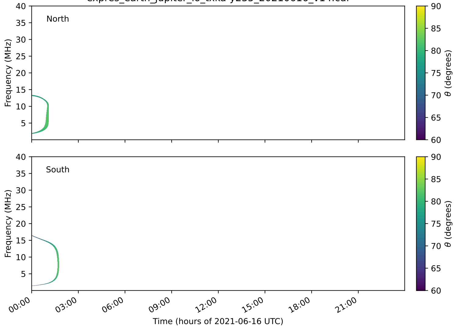
expres_earth_jupiter_io_txka-y235_20210616_v14.cdf
