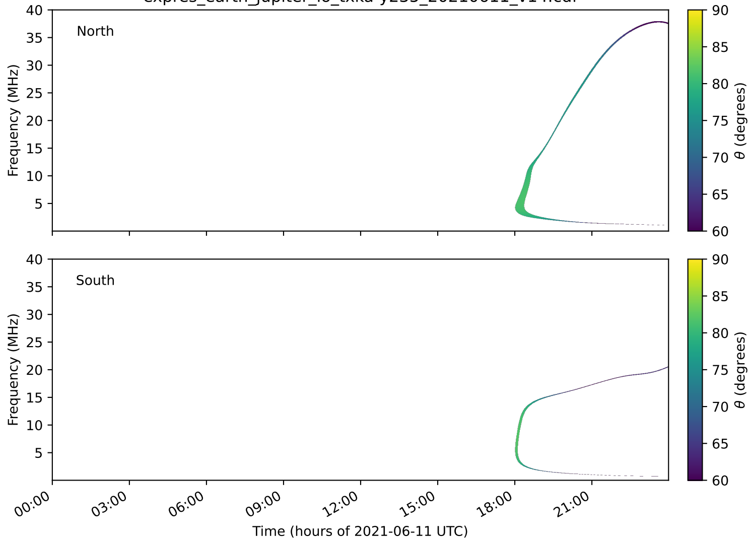
expres_earth_jupiter_io_txka-y235_20210611_v14.cdf
