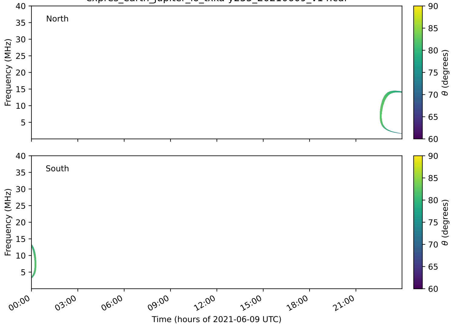
expres_earth_jupiter_io_txka-y235_20210609_v14.cdf
