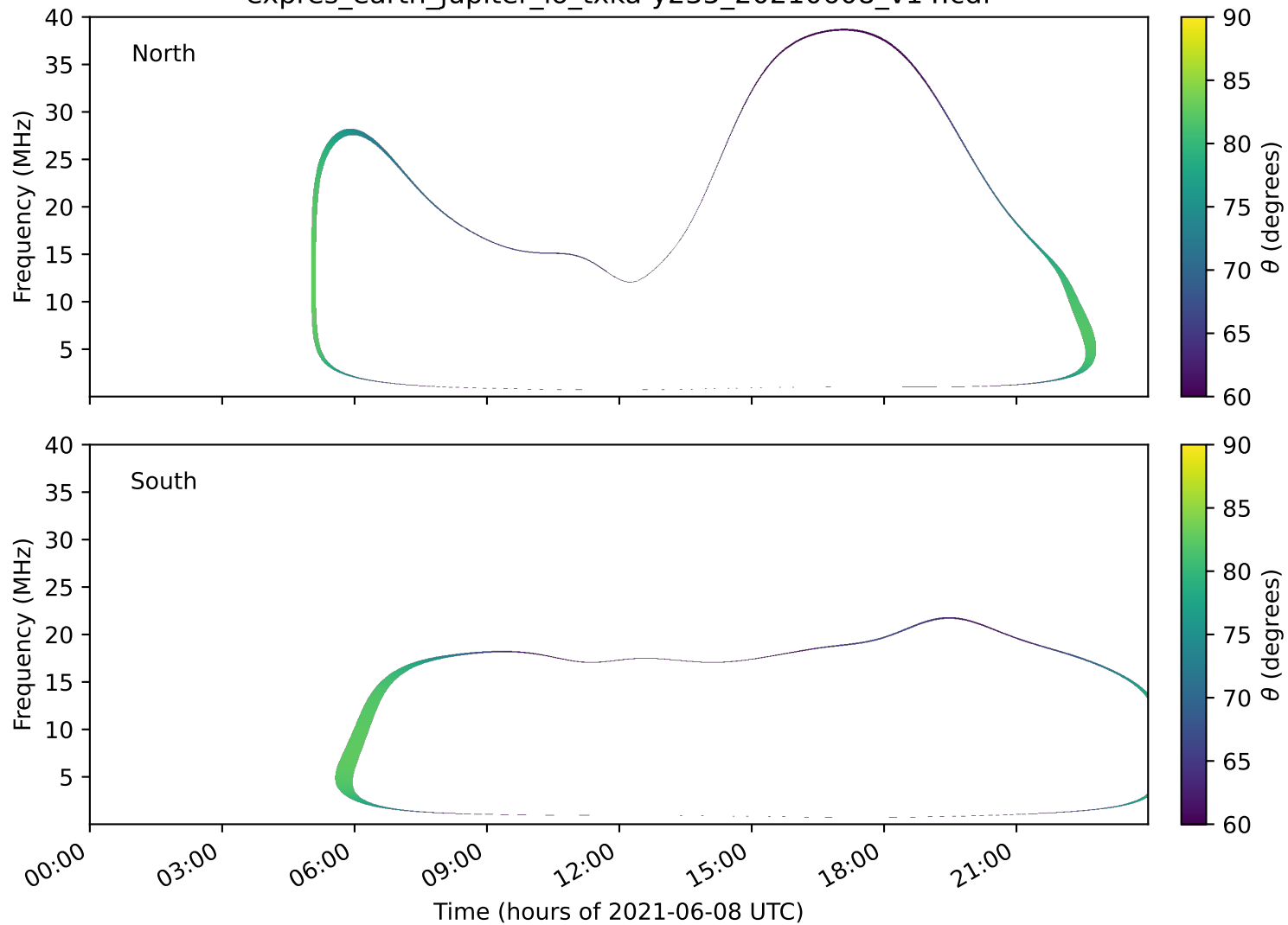
expres_earth_jupiter_io_txka-y235_20210608_v14.cdf
