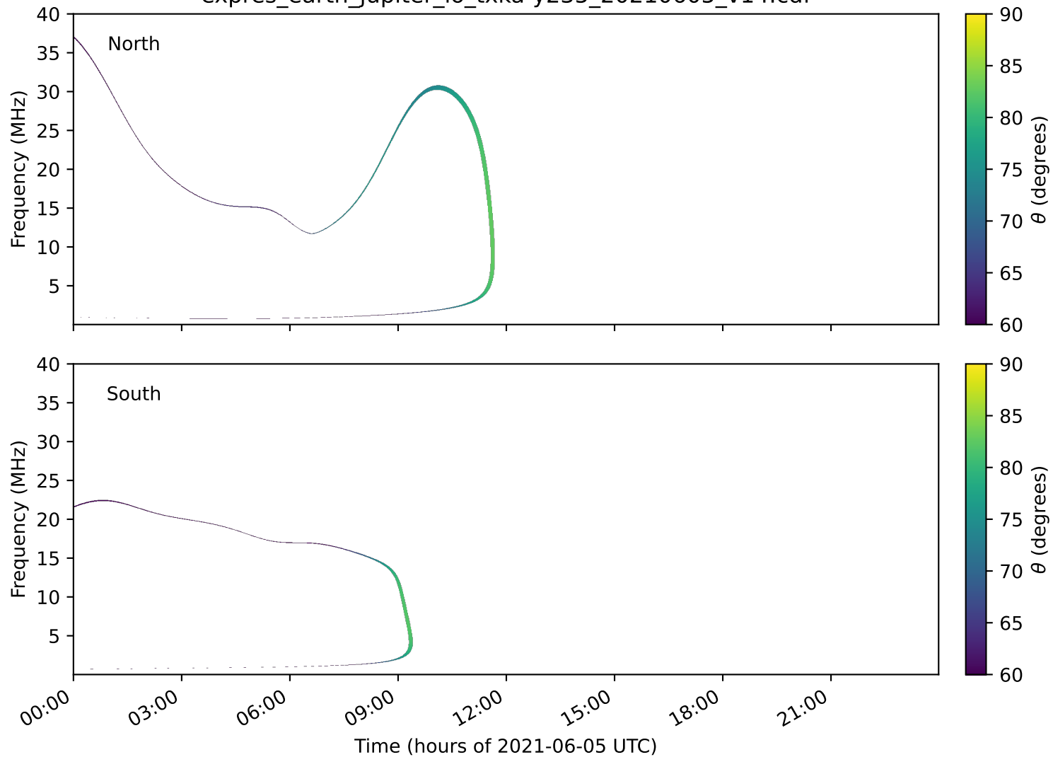
expres_earth_jupiter_io_txka-y235_20210605_v14.cdf
