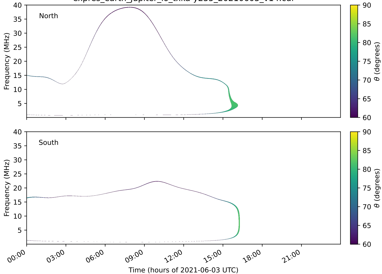
expres_earth_jupiter_io_txka-y235_20210603_v14.cdf
