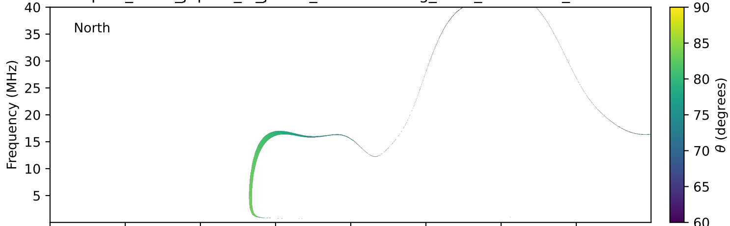
expres_earth_jupiter_io_jrm33_lossc-wid1deg_3kev_20210622_v11.cdf
