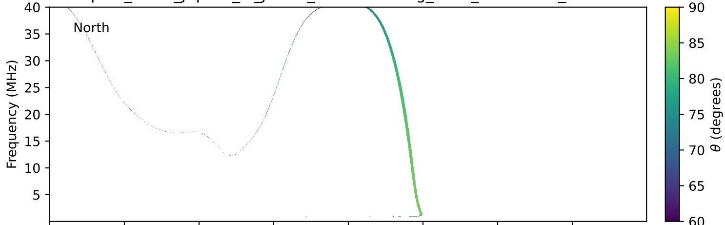
expres_earth_jupiter_io_jrm33_lossc-wid1deg_3kev_20210619_v11.cdf
