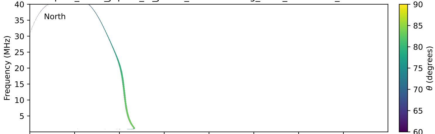
expres_earth_jupiter_io_jrm33_lossc-wid1deg_3kev_20210614_v11.cdf
