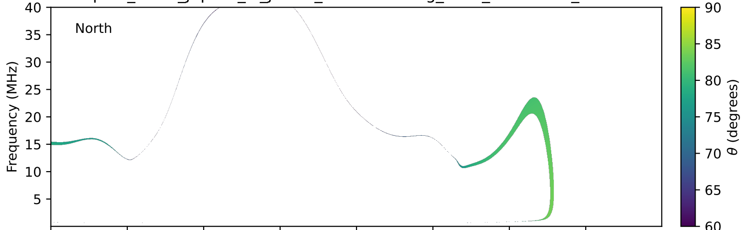
expres_earth_jupiter_io_jrm33_lossc-wid1deg_3kev_20210610_v11.cdf
