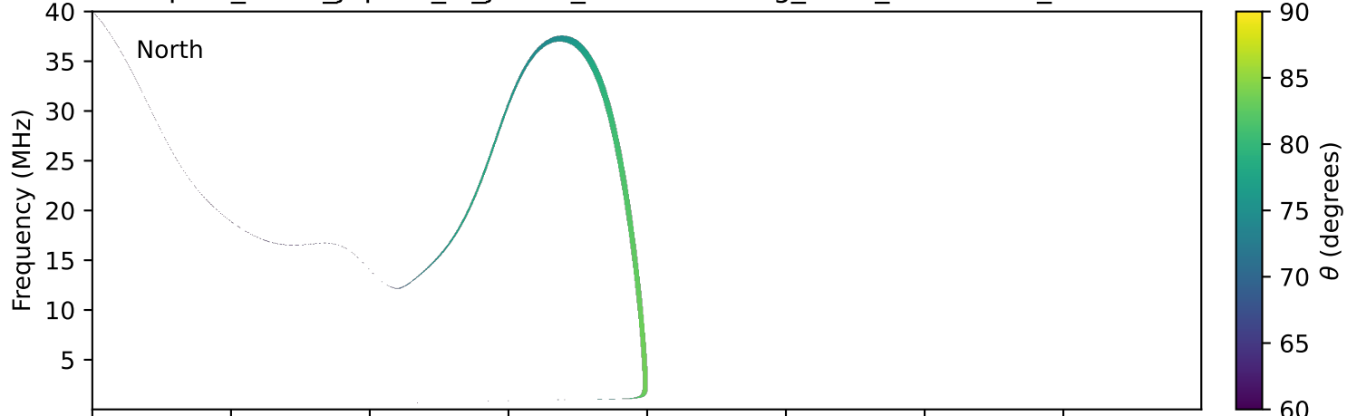
expres_earth_jupiter_io_jrm33_lossc-wid1deg_3kev_20210605_v11.cdf
