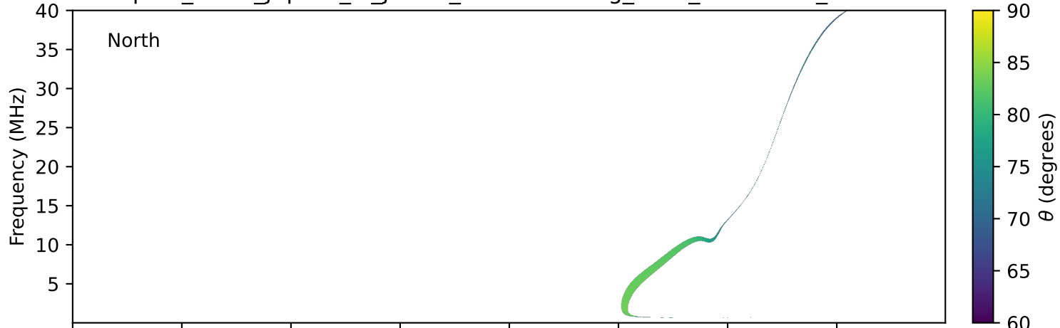
expres_earth_jupiter_io_jrm33_lossc-wid1deg_3kev_20210604_v11.cdf
