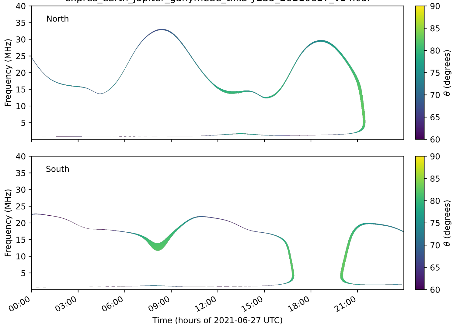
expres_earth_jupiter_ganymede_txka-y235_20210627_v14.cdf
