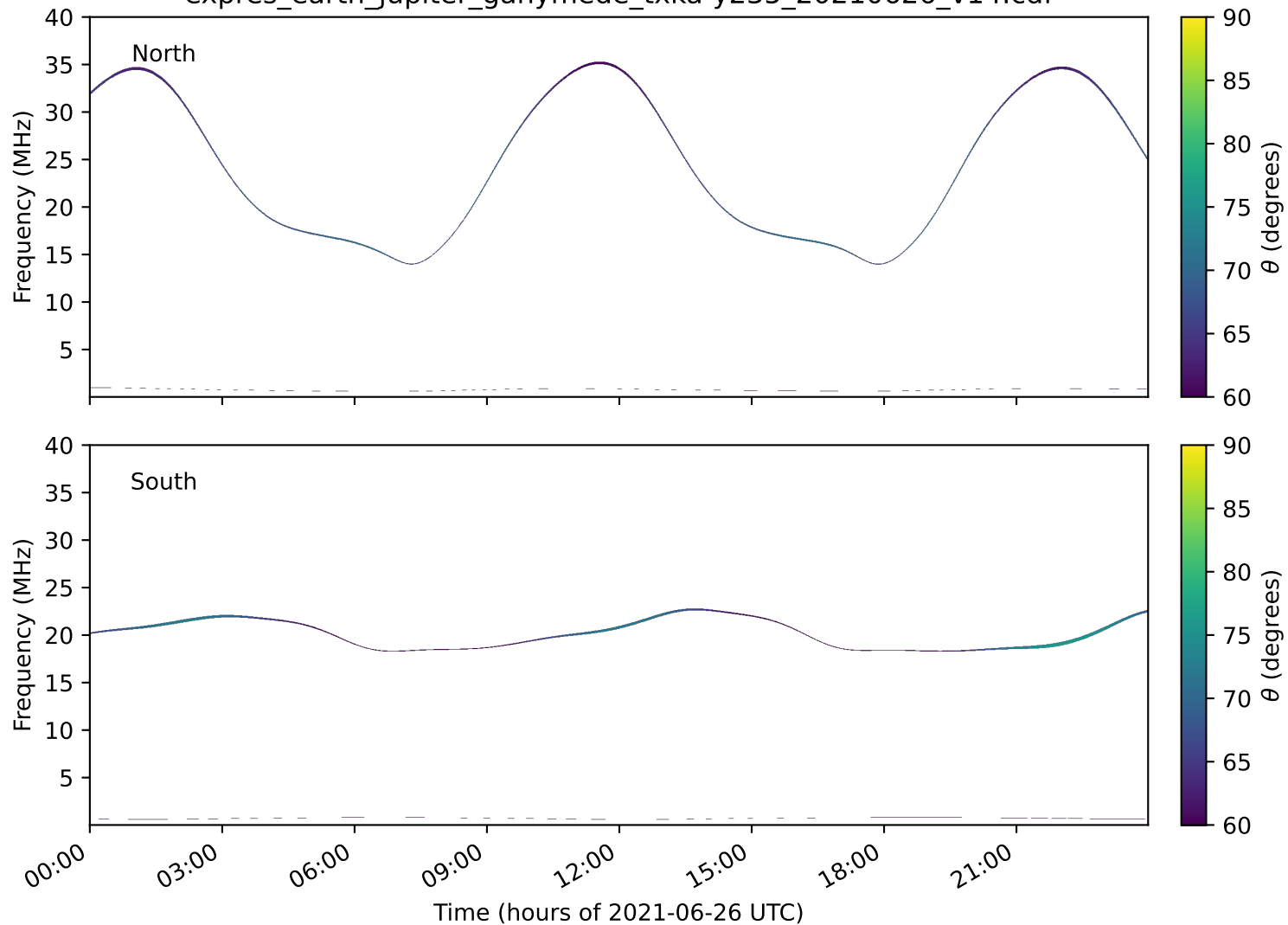
expres_earth_jupiter_ganymede_txka-y235_20210626_v14.cdf
