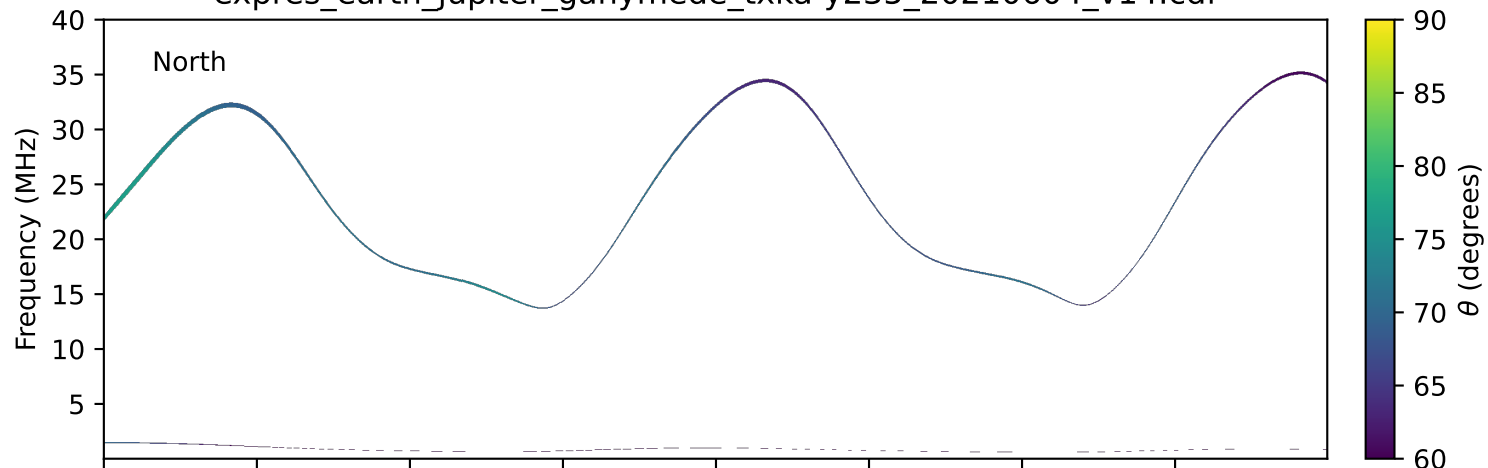
expres_earth_jupiter_ganymede_txka-y235_20210604_v14.cdf
