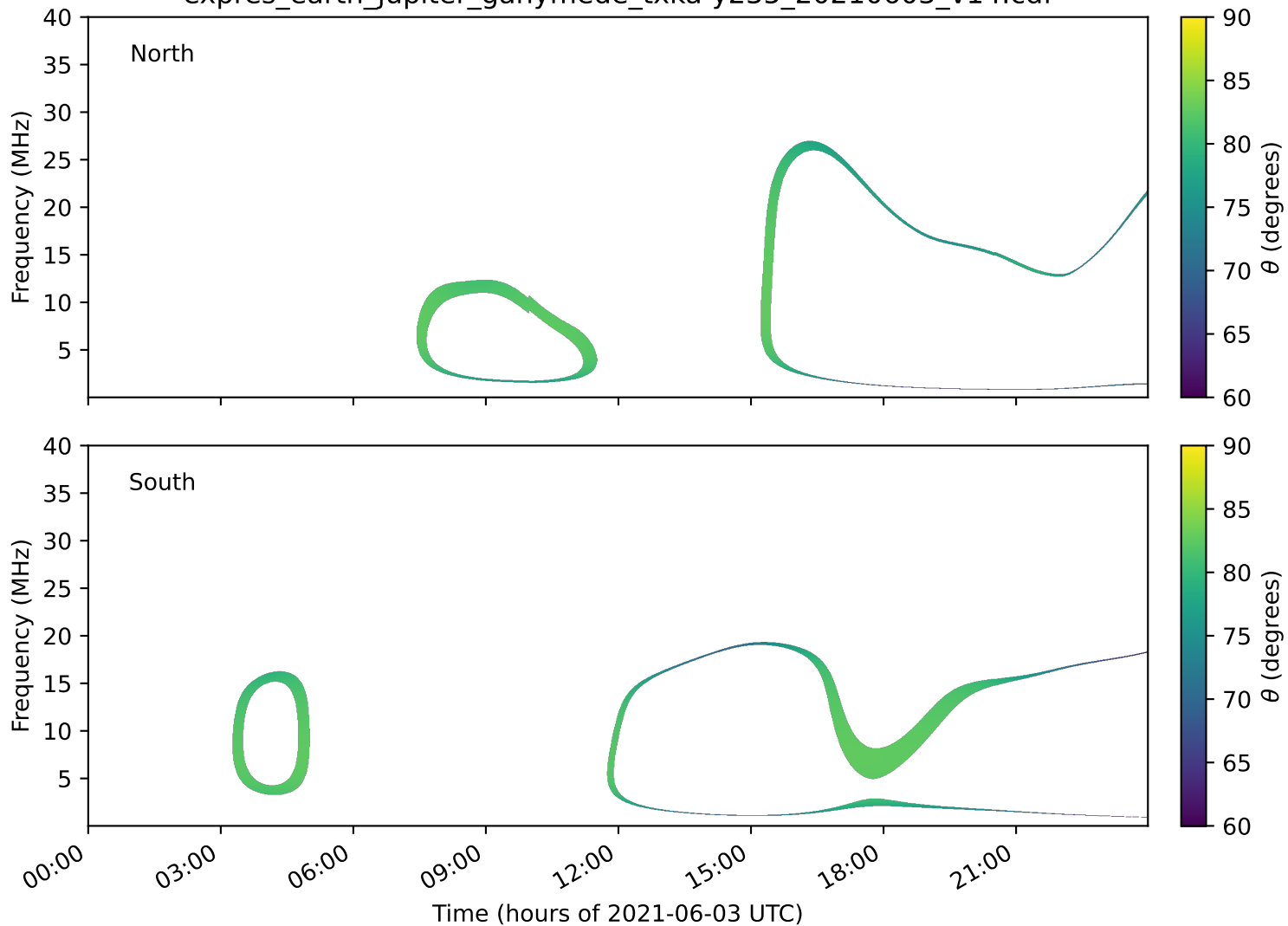
expres_earth_jupiter_ganymede_txka-y235_20210603_v14.cdf
