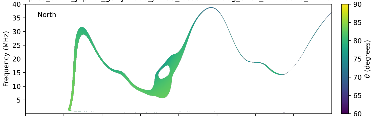
expres_earth_jupiter_ganymede_jrm33_lossc-wid1deg_3kev_20210625_v11.cdf
