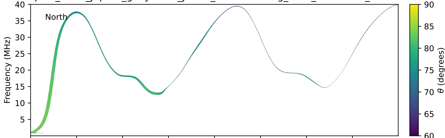
expres_earth_jupiter_ganymede_jrm33_lossc-wid1deg_3kev_20210611_v11.cdf
