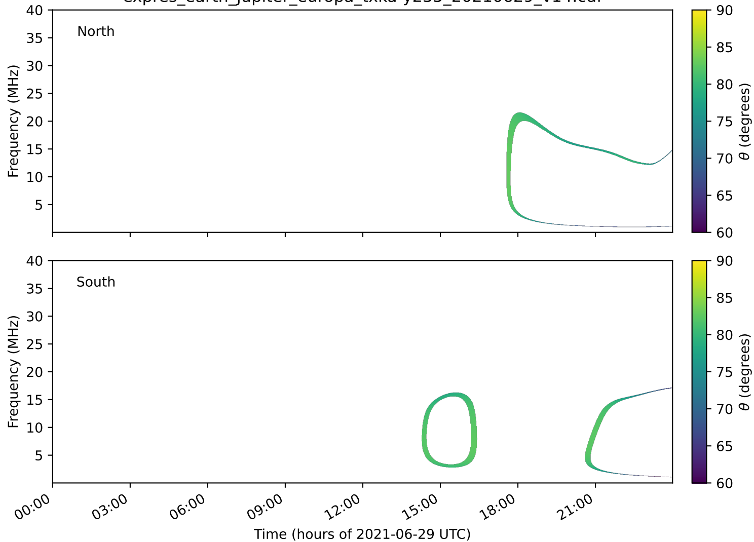
expres_earth_jupiter_europa_txka-y235_20210629_v14.cdf
