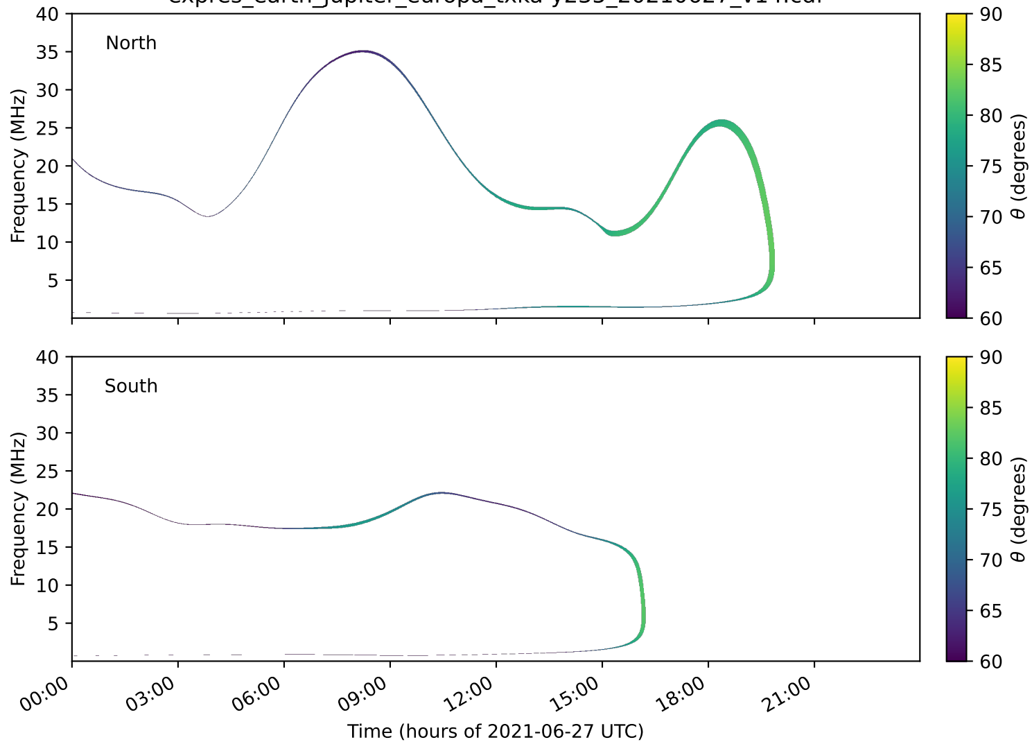
expres_earth_jupiter_europa_txka-y235_20210627_v14.cdf
