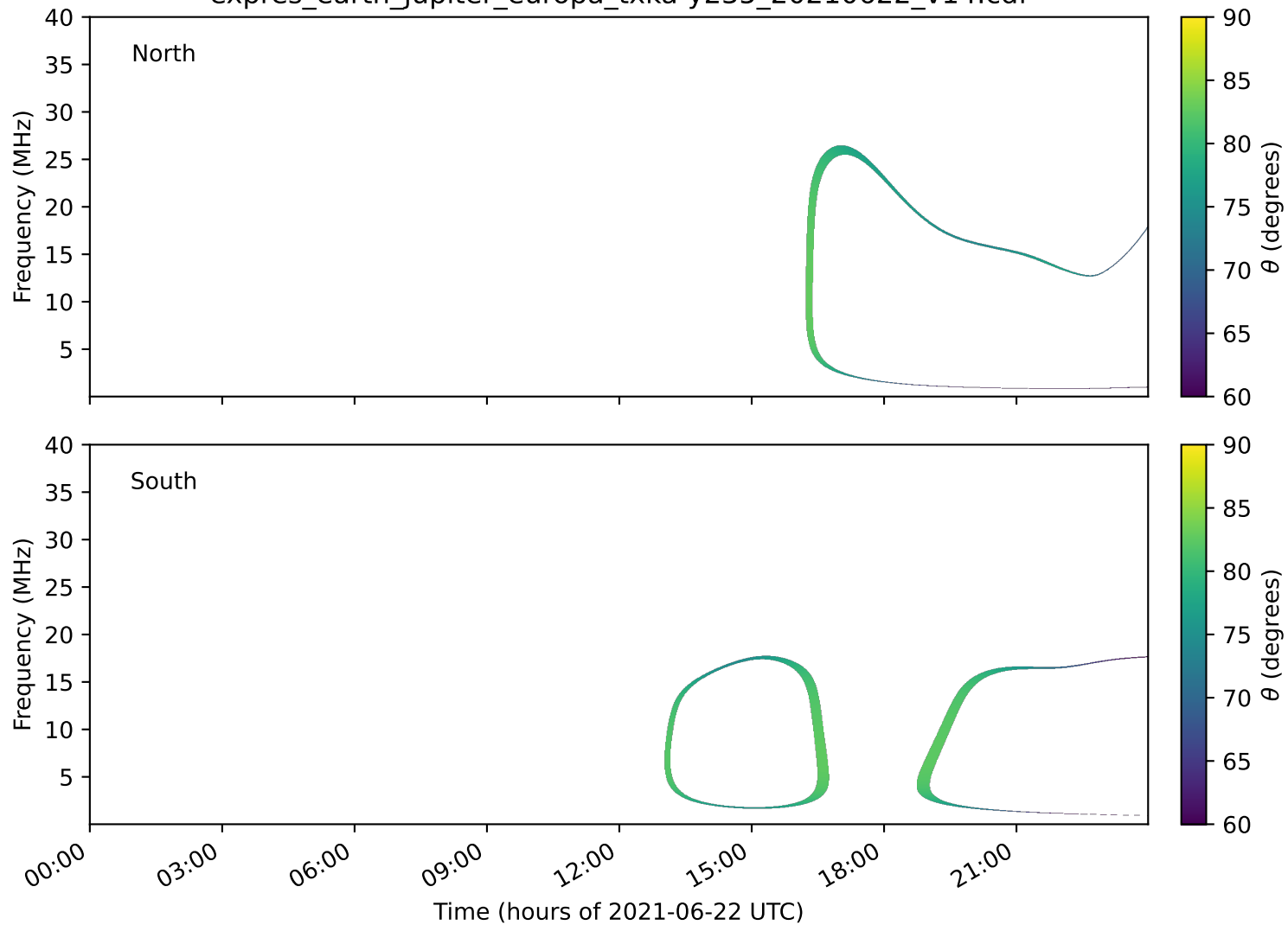
expres_earth_jupiter_europa_txka-y235_20210622_v14.cdf
