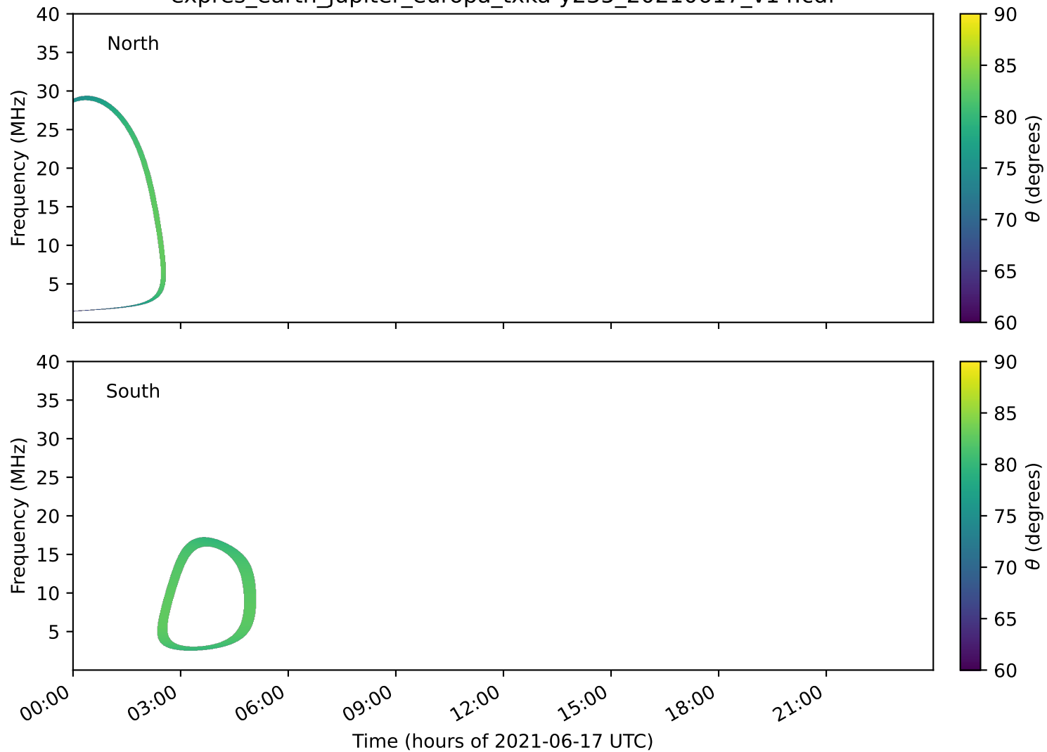
expres_earth_jupiter_europa_txka-y235_20210617_v14.cdf
