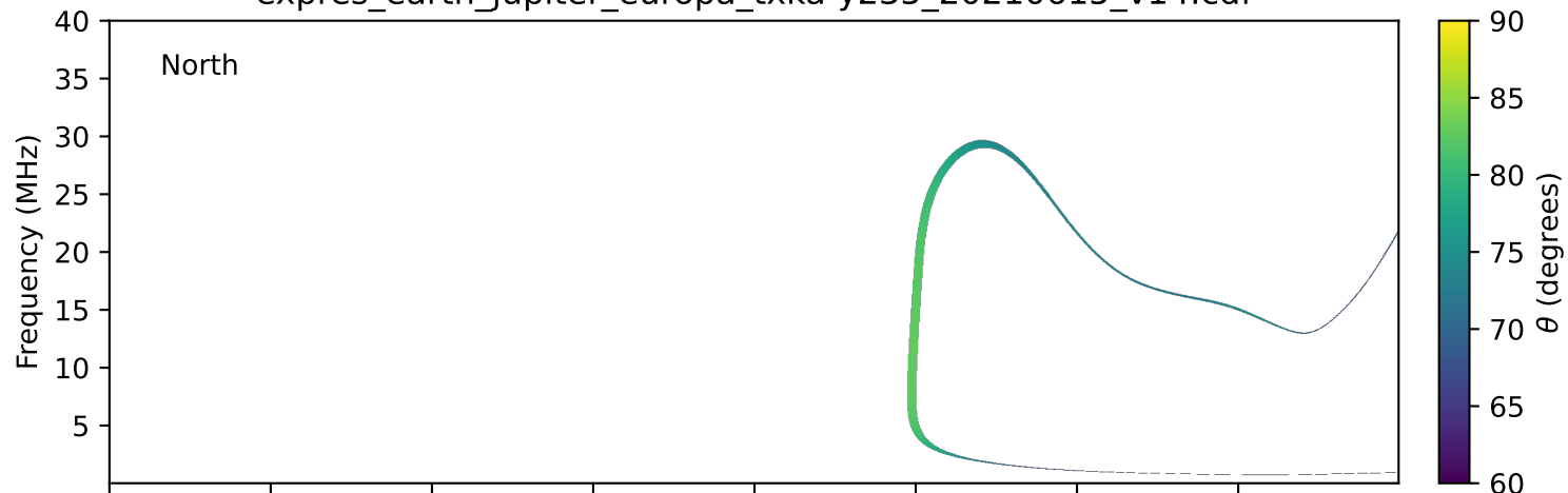
expres_earth_jupiter_europa_txka-y235_20210615_v14.cdf
