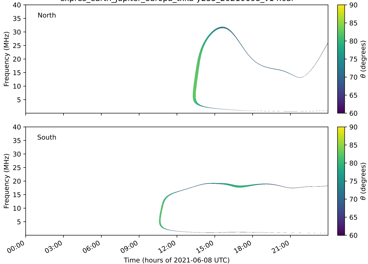
expres_earth_jupiter_europa_txka-y235_20210608_v14.cdf
