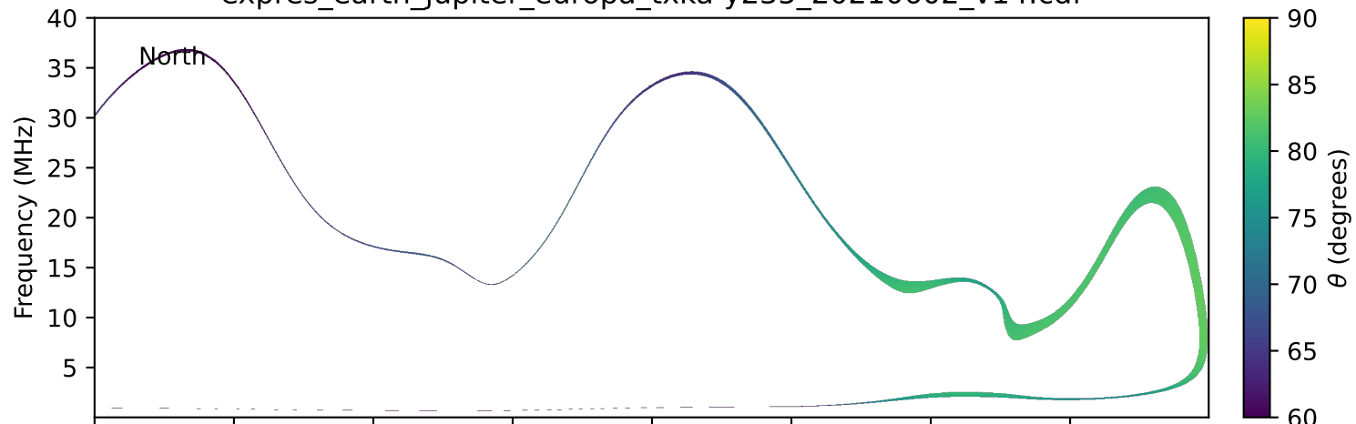
expres_earth_jupiter_europa_txka-y235_20210602_v14.cdf
