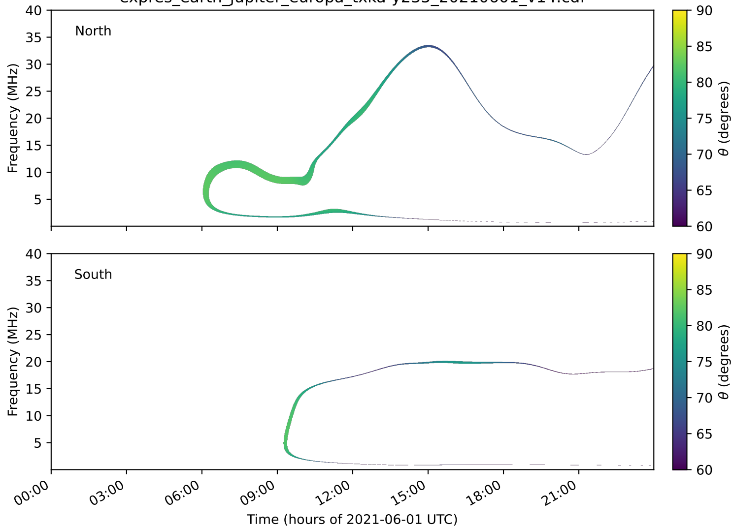
expres_earth_jupiter_europa_txka-y235_20210601_v14.cdf
