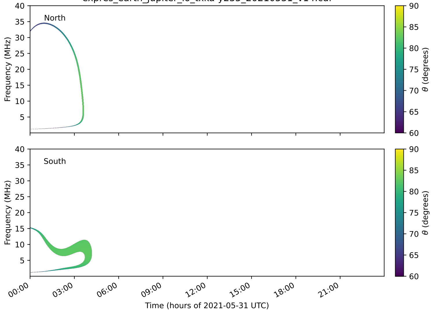
expres_earth_jupiter_io_txka-y235_20210531_v14.cdf
