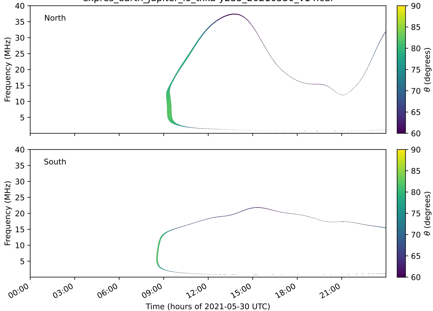
expres_earth_jupiter_io_txka-y235_20210530_v14.cdf
