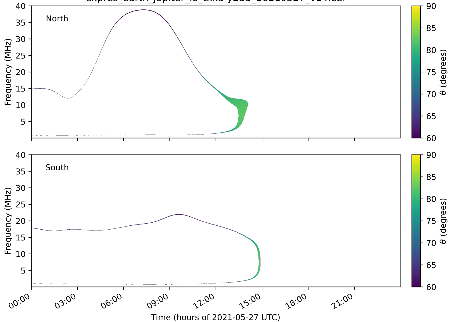
expres_earth_jupiter_io_txka-y235_20210527_v14.cdf
