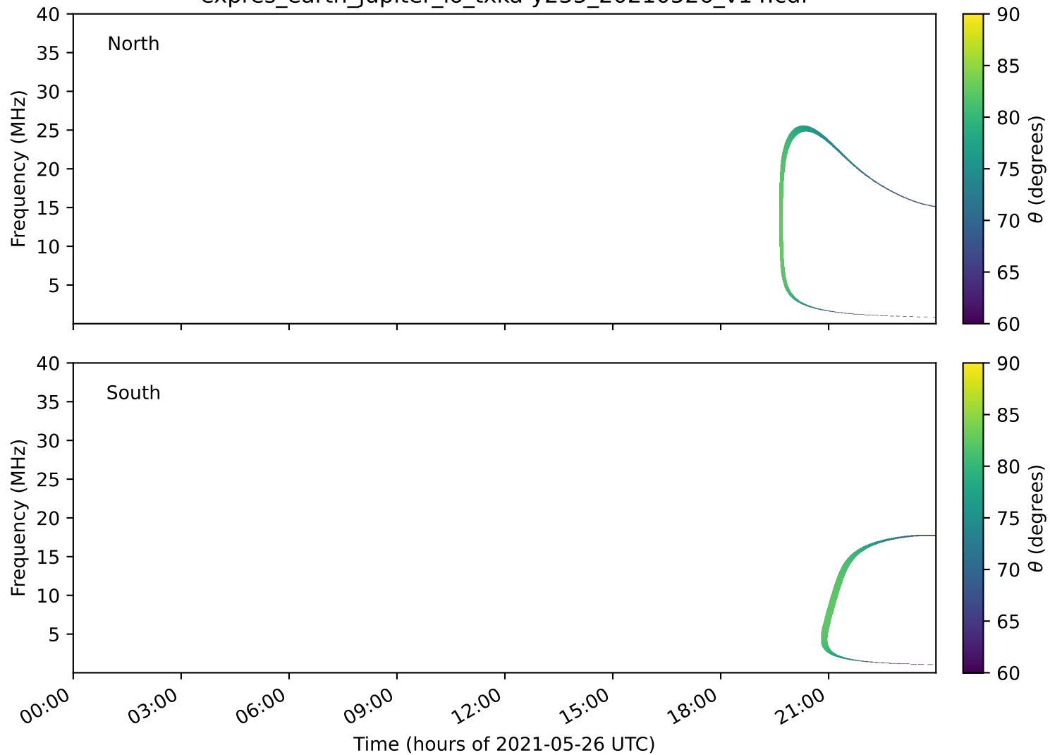
expres_earth_jupiter_io_txka-y235_20210526_v14.cdf
