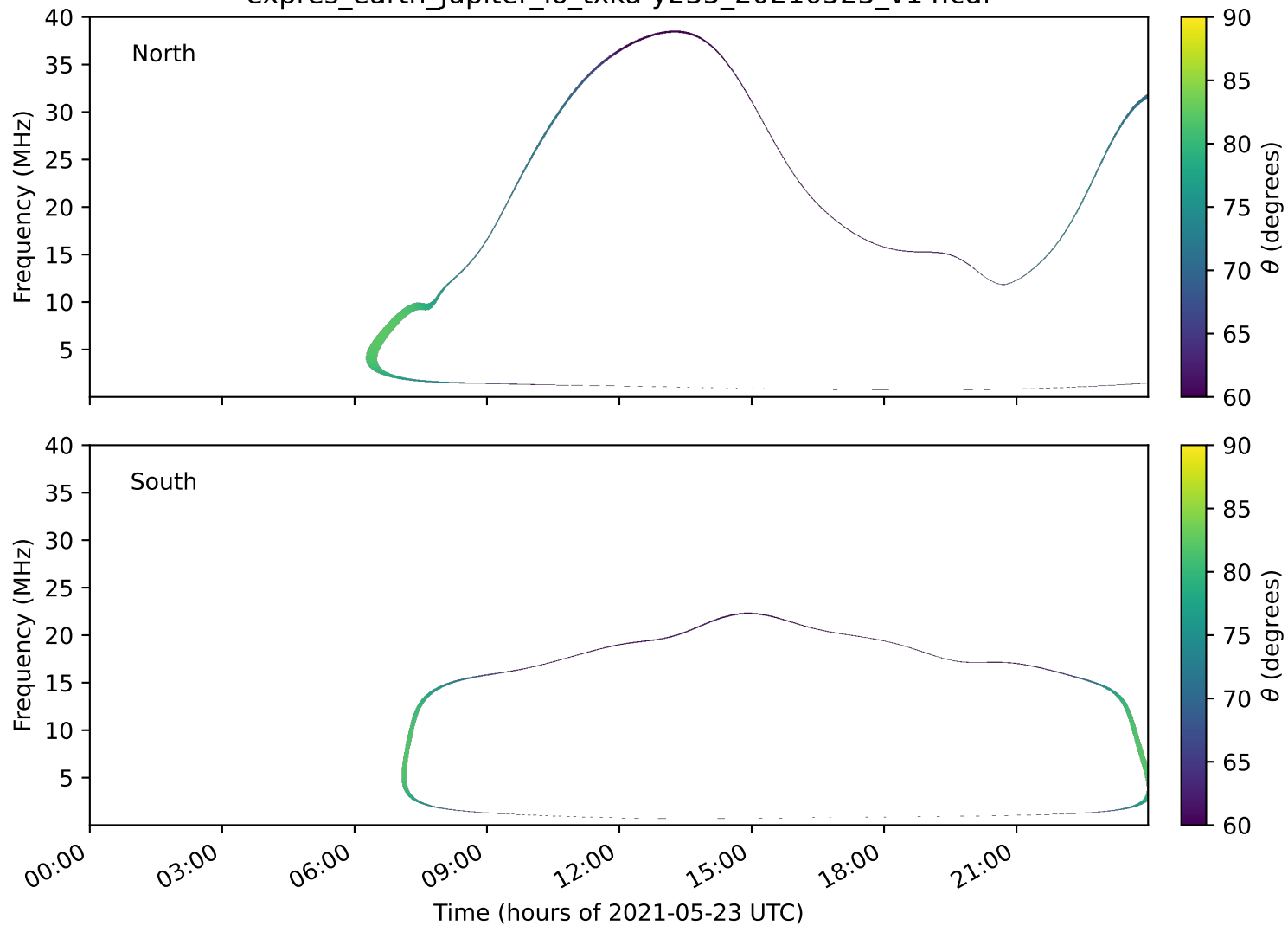
expres_earth_jupiter_io_txka-y235_20210523_v14.cdf
