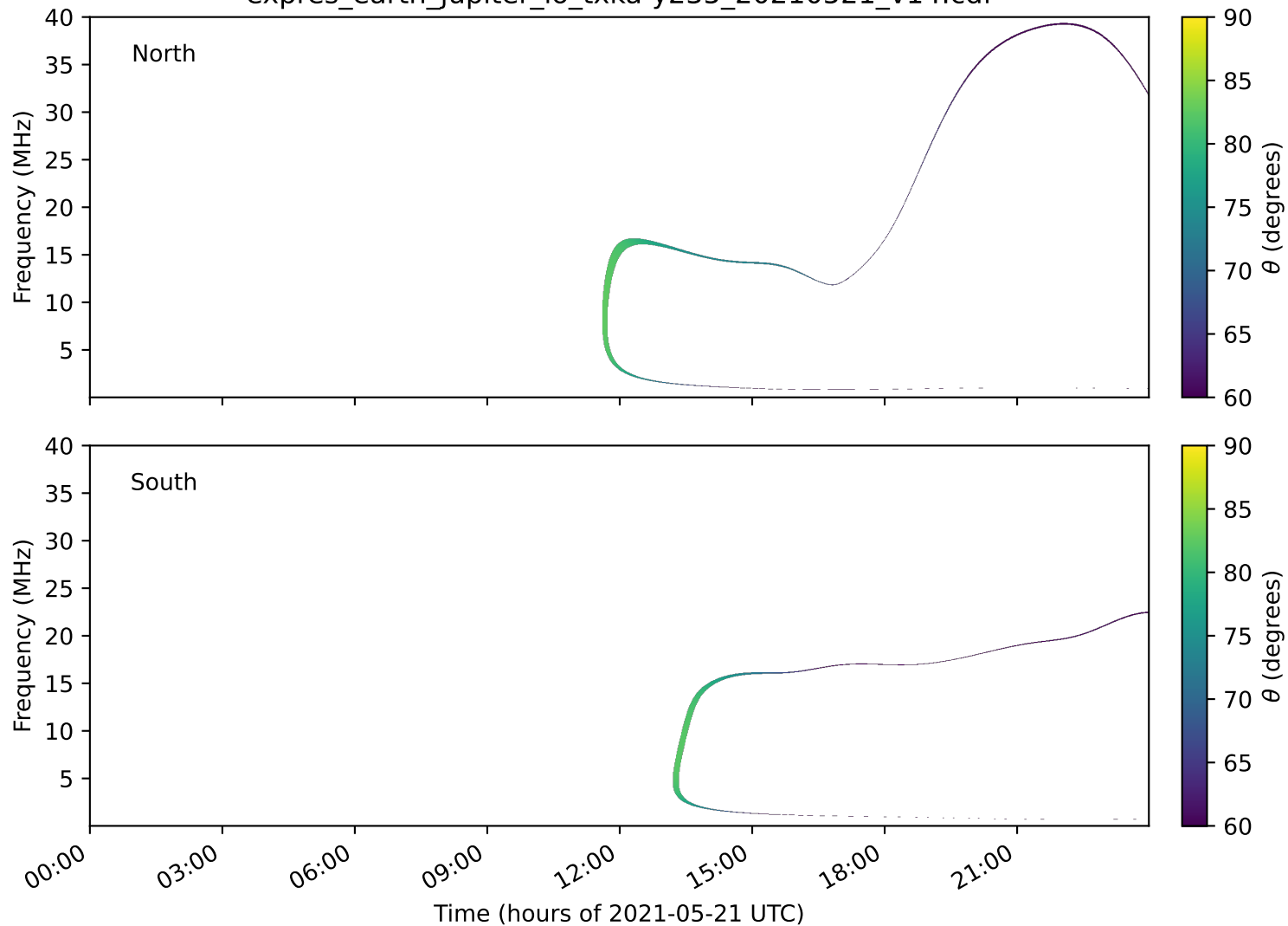
expres_earth_jupiter_io_txka-y235_20210521_v14.cdf
