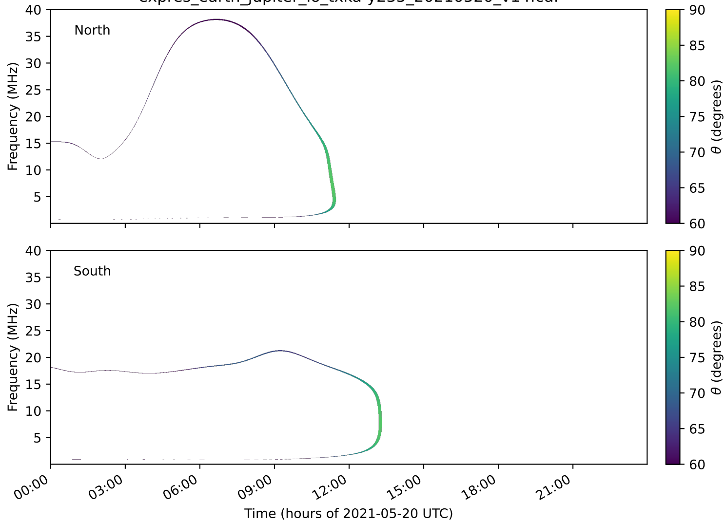
expres_earth_jupiter_io_txka-y235_20210520_v14.cdf
