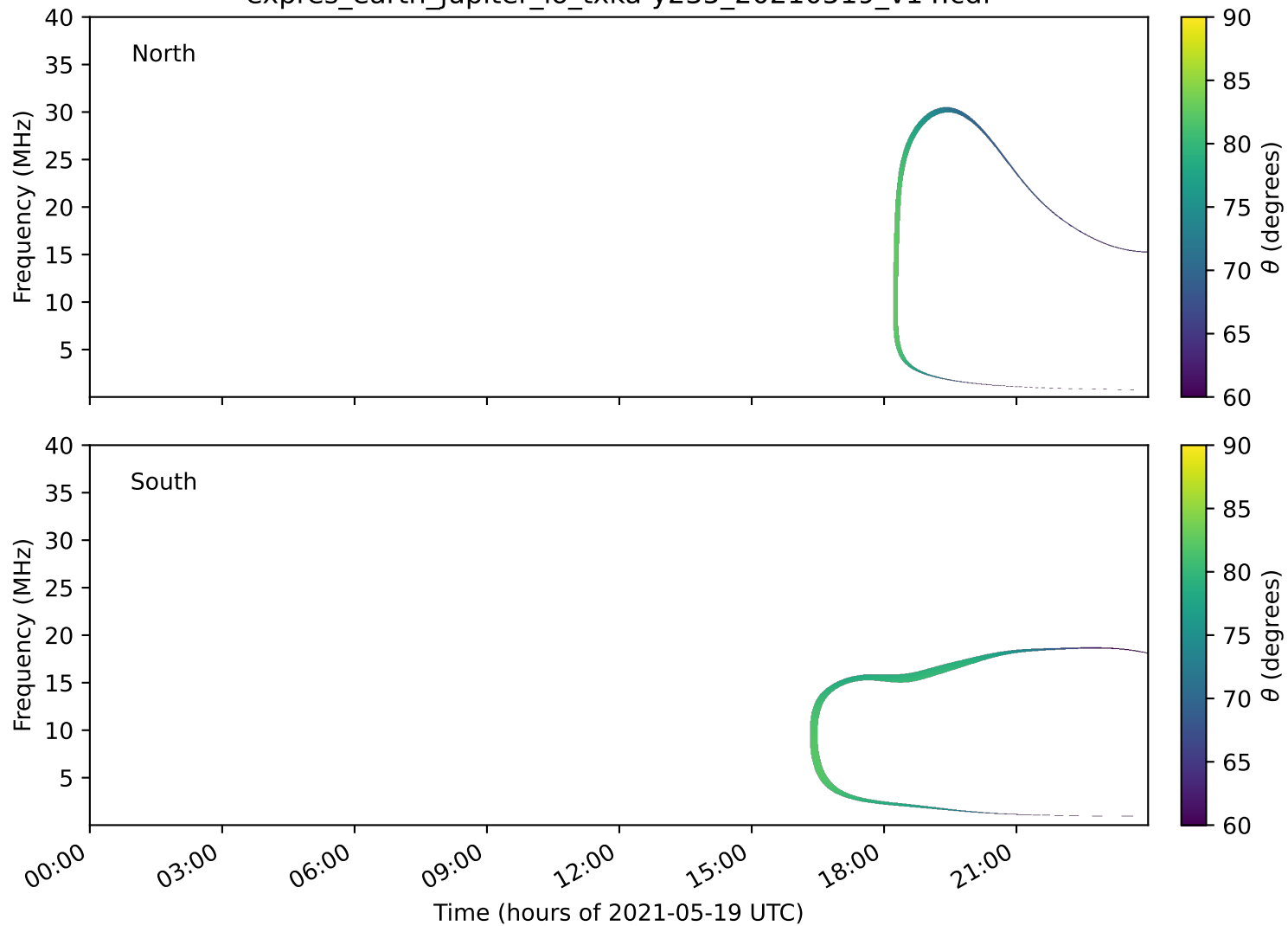
expres_earth_jupiter_io_txka-y235_20210519_v14.cdf
