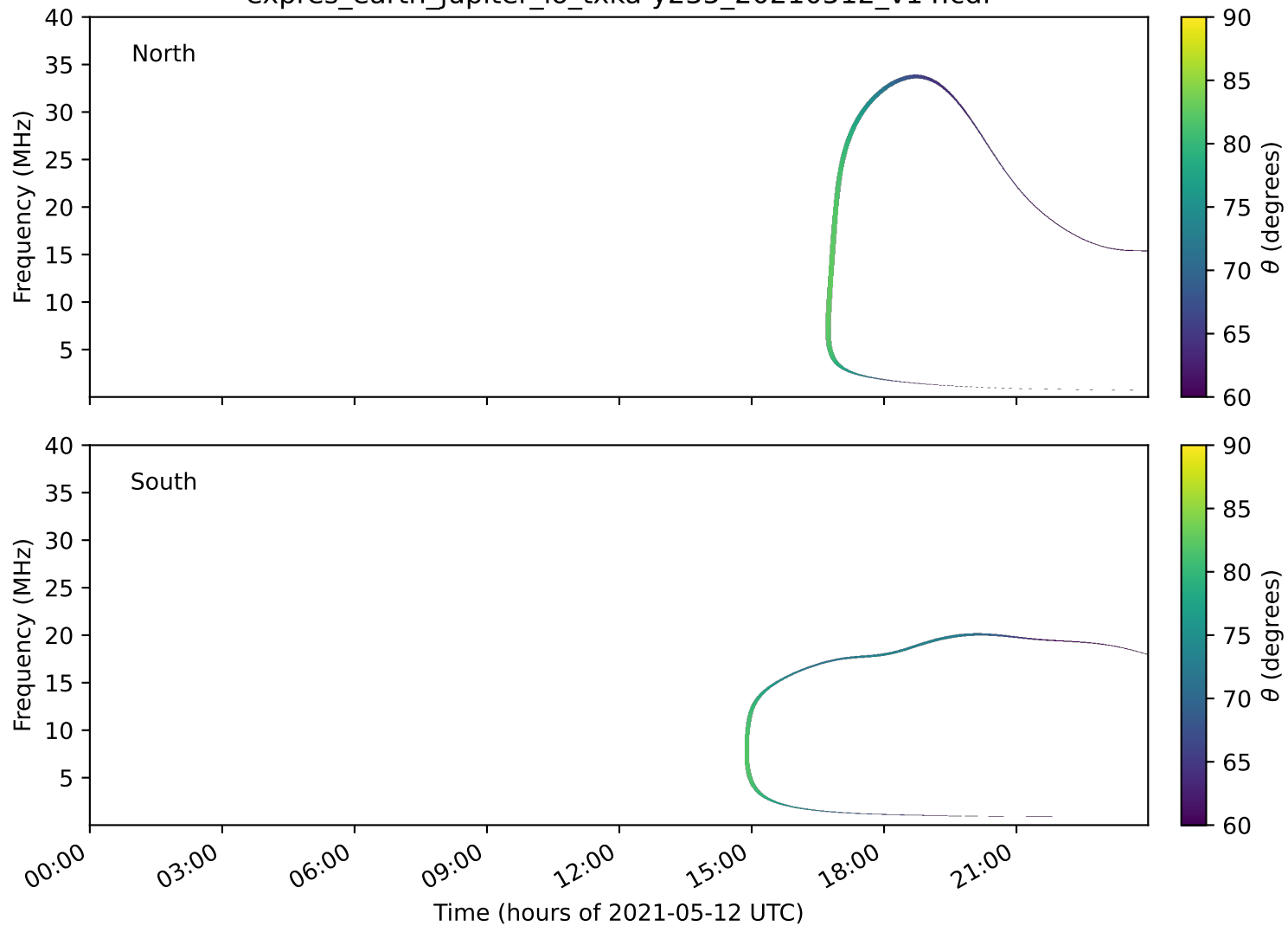
expres_earth_jupiter_io_txka-y235_20210512_v14.cdf
