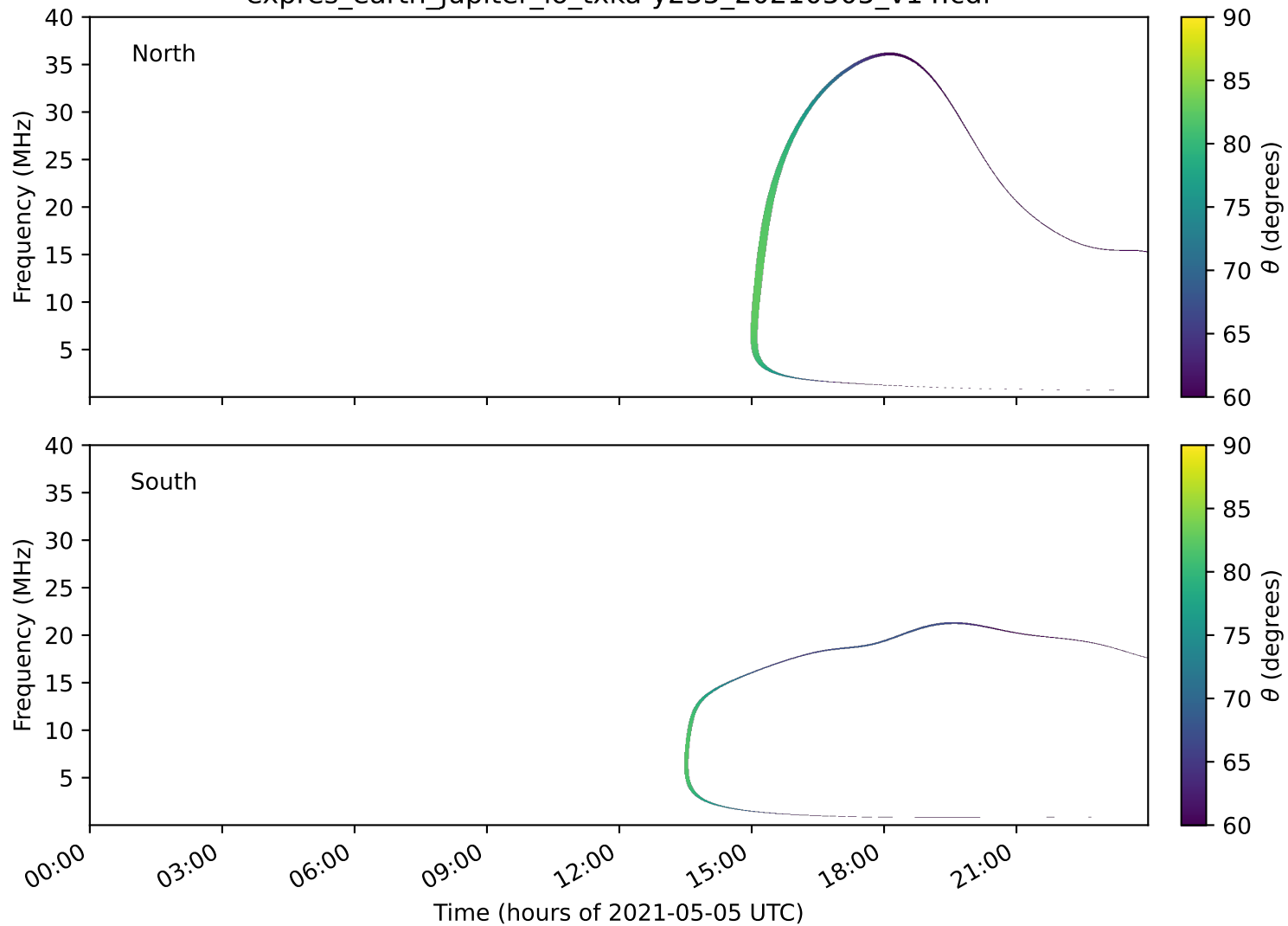
expres_earth_jupiter_io_txka-y235_20210505_v14.cdf
