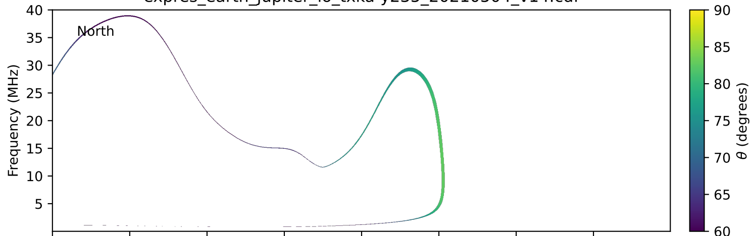
expres_earth_jupiter_io_txka-y235_20210504_v14.cdf
