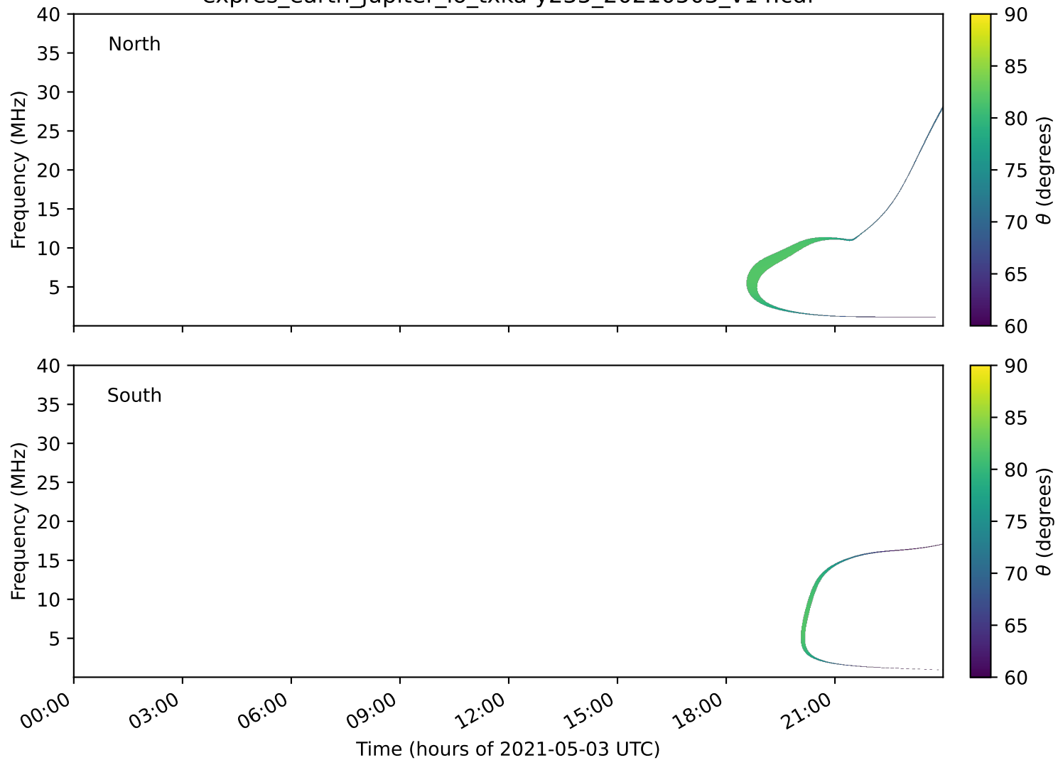
expres_earth_jupiter_io_txka-y235_20210503_v14.cdf
