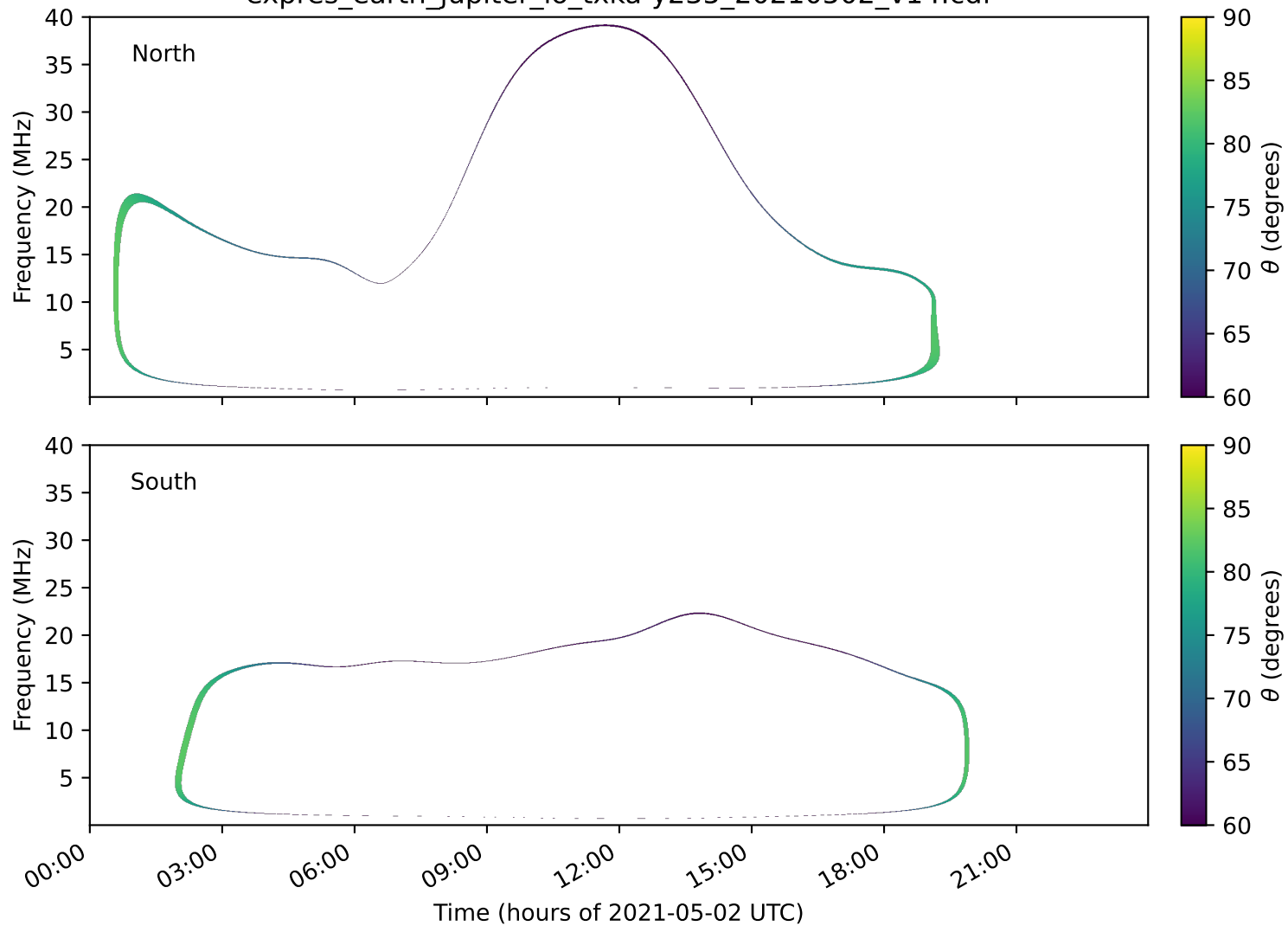
expres_earth_jupiter_io_txka-y235_20210502_v14.cdf
