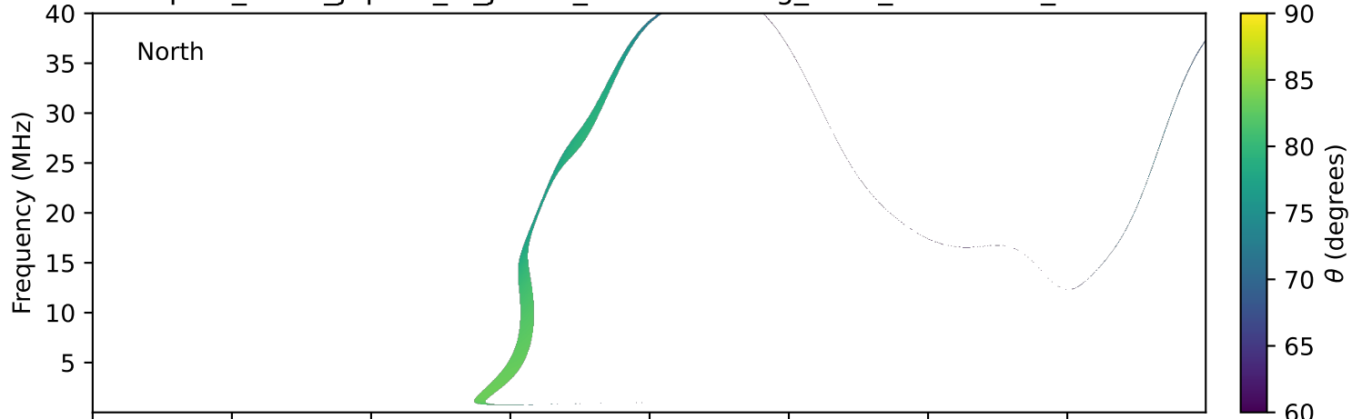
expres_earth_jupiter_io_jrm33_lossc-wid1deg_3kev_20210530_v11.cdf
