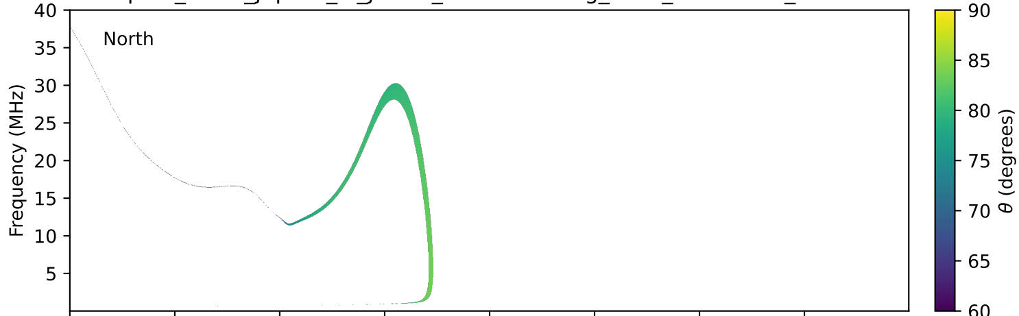
expres_earth_jupiter_io_jrm33_lossc-wid1deg_3kev_20210529_v11.cdf
