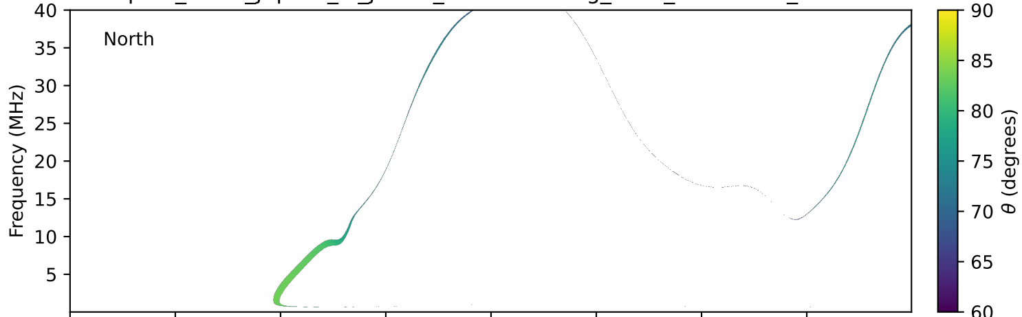
expres_earth_jupiter_io_jrm33_lossc-wid1deg_3kev_20210523_v11.cdf
