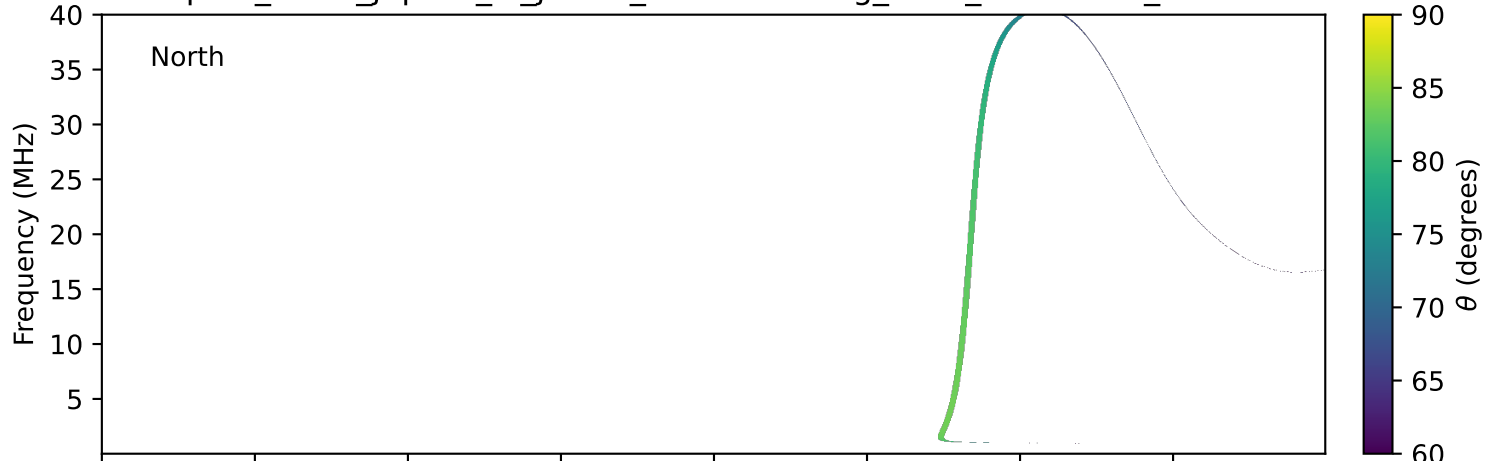
expres_earth_jupiter_io_jrm33_lossc-wid1deg_3kev_20210512_v11.cdf
