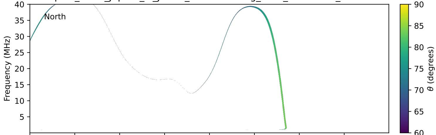
expres_earth_jupiter_io_jrm33_lossc-wid1deg_3kev_20210511_v11.cdf
