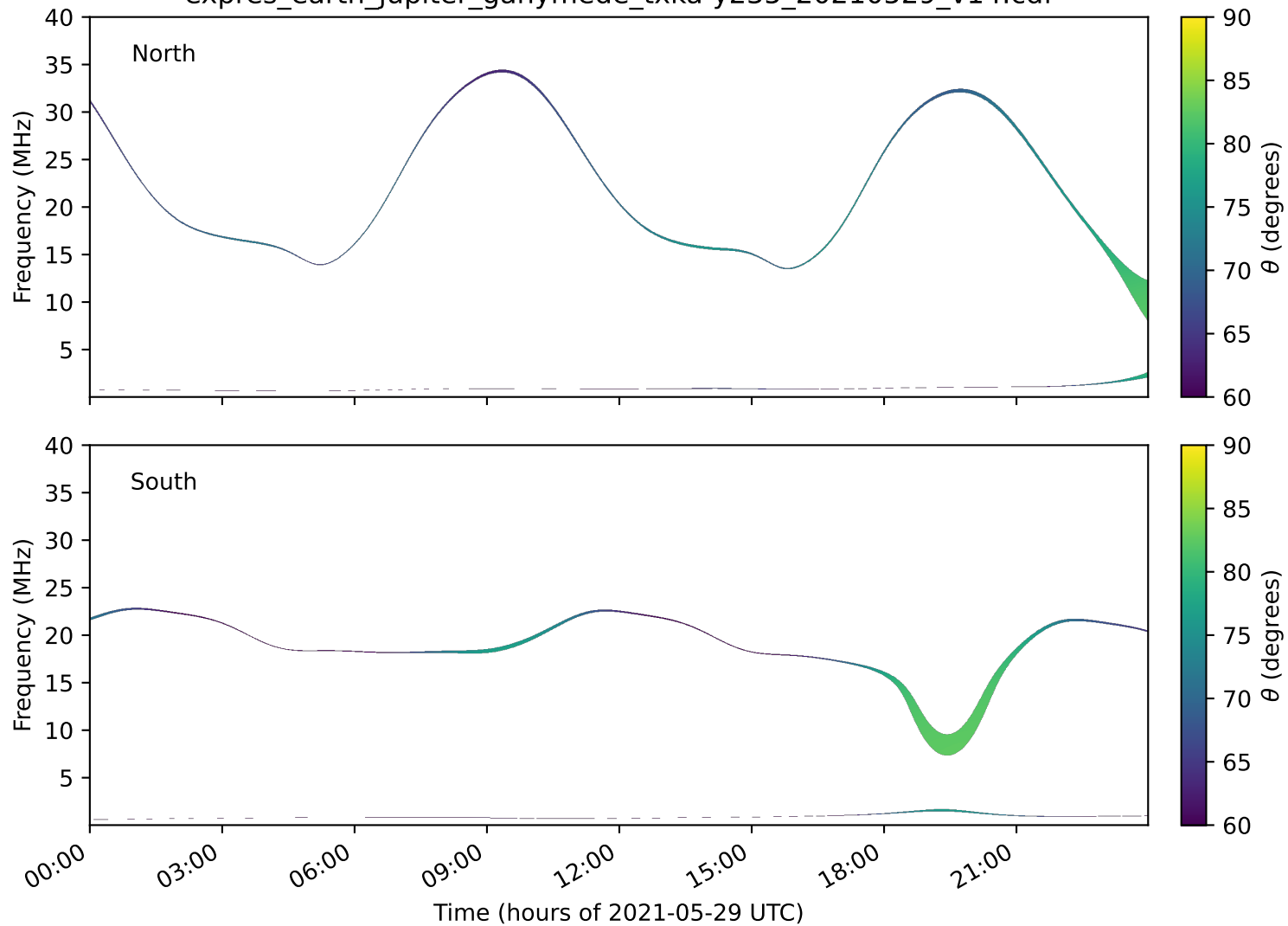
expres_earth_jupiter_ganymede_txka-y235_20210529_v14.cdf
