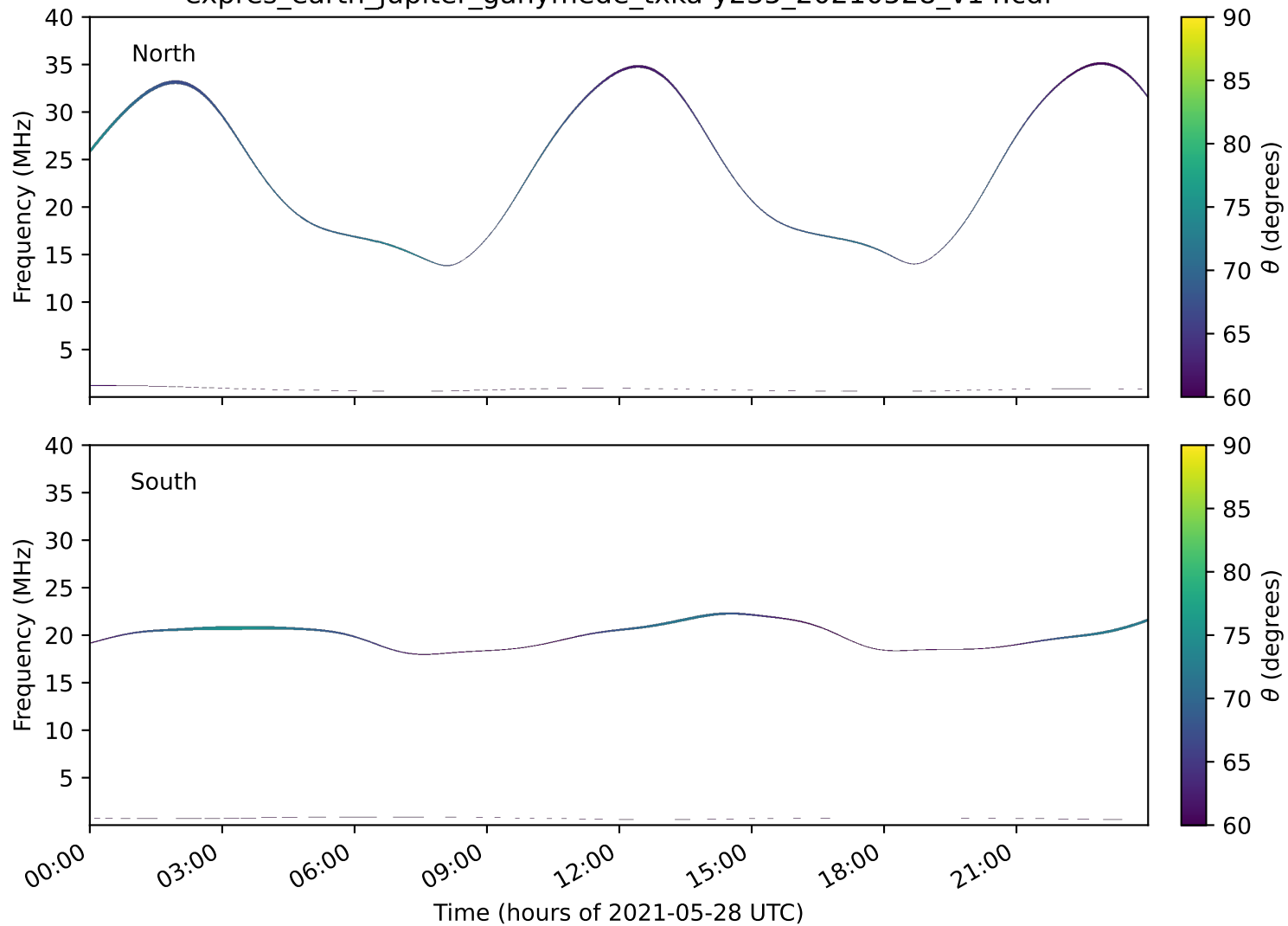
expres_earth_jupiter_ganymede_txka-y235_20210528_v14.cdf
