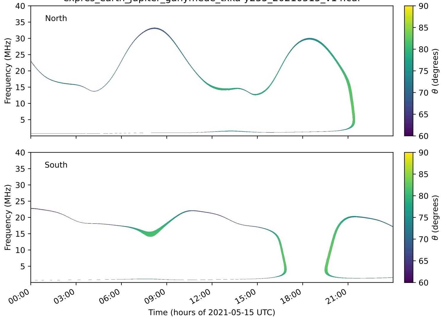
expres_earth_jupiter_ganymede_txka-y235_20210515_v14.cdf
