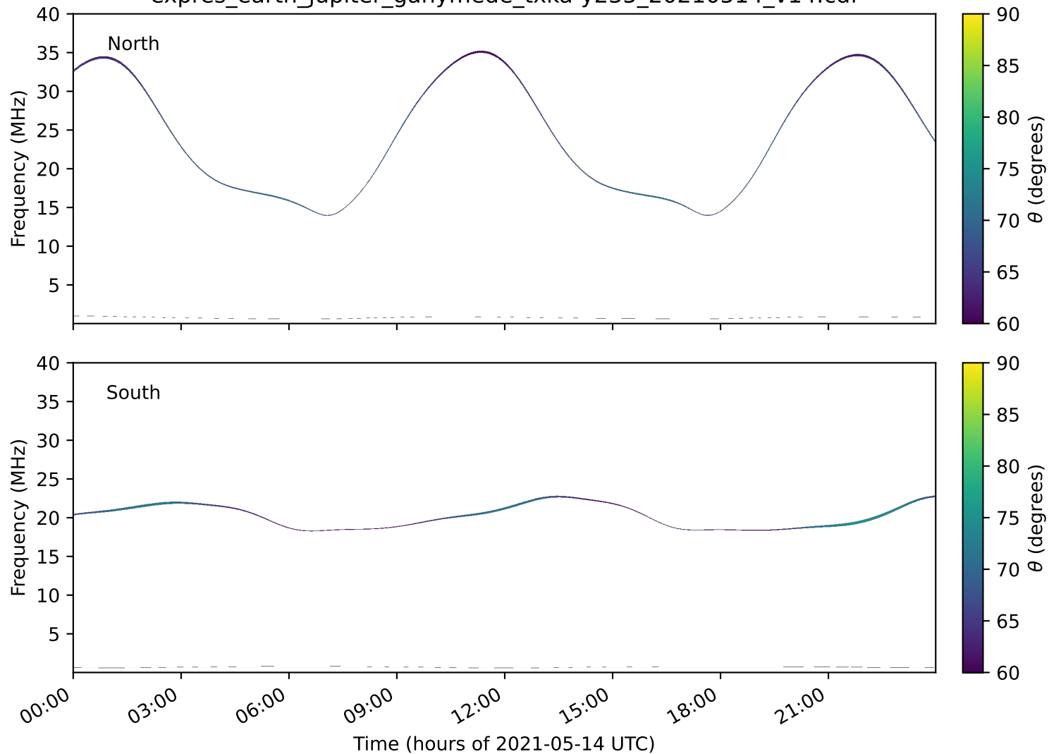
expres_earth_jupiter_ganymede_txka-y235_20210514_v14.cdf
