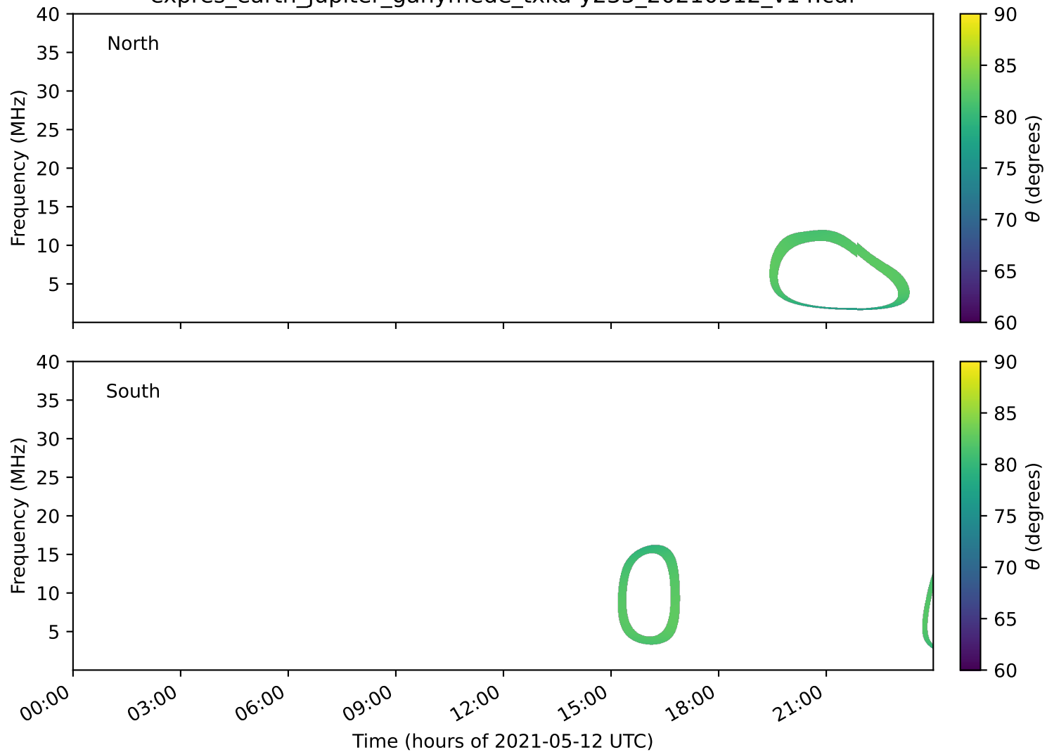
expres_earth_jupiter_ganymede_txka-y235_20210512_v14.cdf
